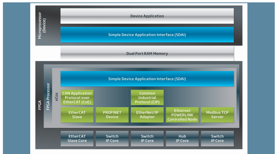
Figure 1: Cost-efficient, flexible and future-proof: FPGAs in field devices support different Industrial Ethernet protocols.
