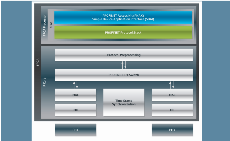
Figure 2: Structure of the FPGA-based PROFINET IRT implementation.
